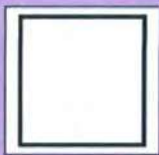
square n square adj
